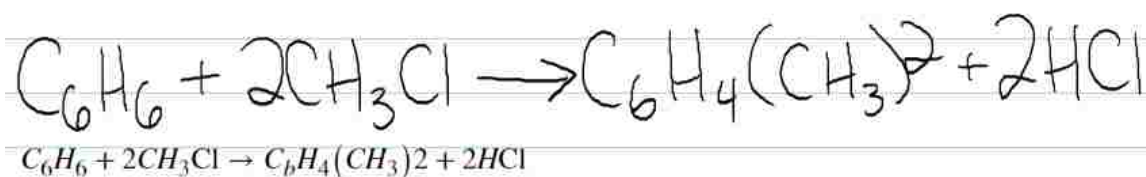
Figure 4.20: Example of a WOZ Recognizer's sketch using a stoichiometric equation. Two errors are present in the recognition, a 6 is changed to a b and a 2 is no longer a superscript.
